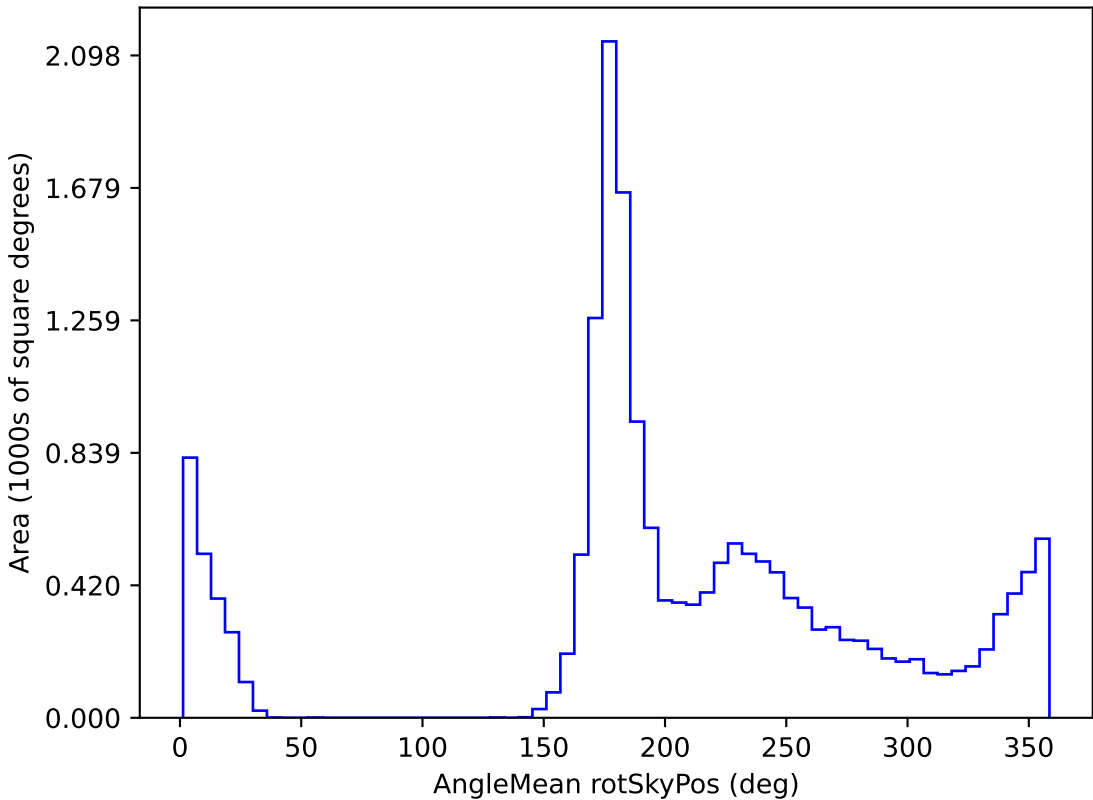
weather_cloudso1v3.4_10yrs WFD r band: AngleMean rotSkyPos
