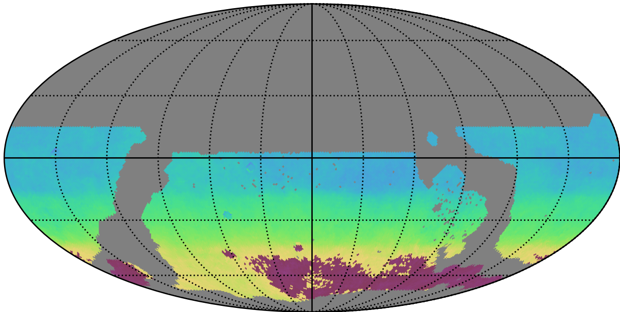
weather_cloudso1v3.4_10yrs WFD i band: AngleMean rotSkyPos
