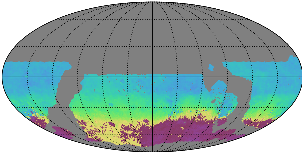
weather_cloudso1v3.4_10yrs WFD g band: AngleMean rotSkyPos
