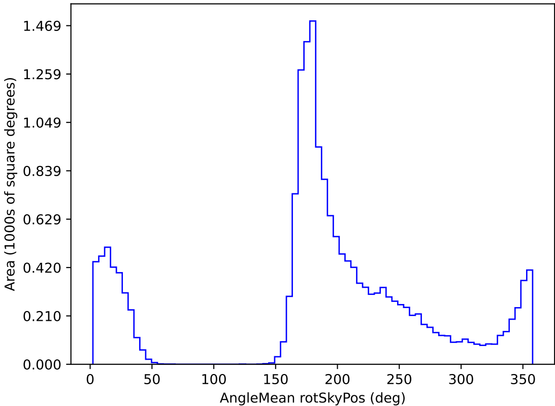
weather_cloudso1v3.4_10yrs WFD g band: AngleMean rotSkyPos
