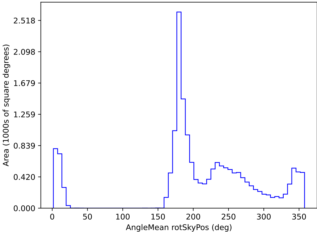
weather_cloudso1v3.4_10yrs WFD all bands: AngleMean rotSkyPos
