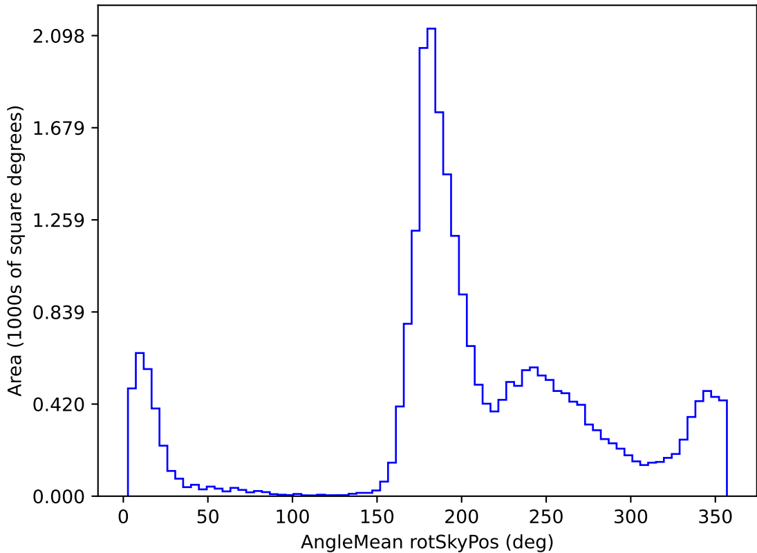
weather_cloudso1v3.4_10yrs All sky z band: AngleMean rotSkyPos
