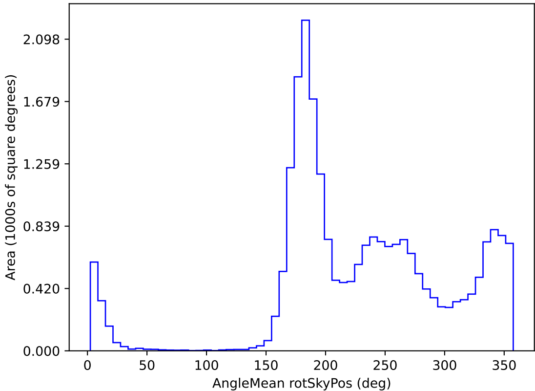
weather_cloudso1v3.4_10yrs All sky y band: AngleMean rotSkyPos
