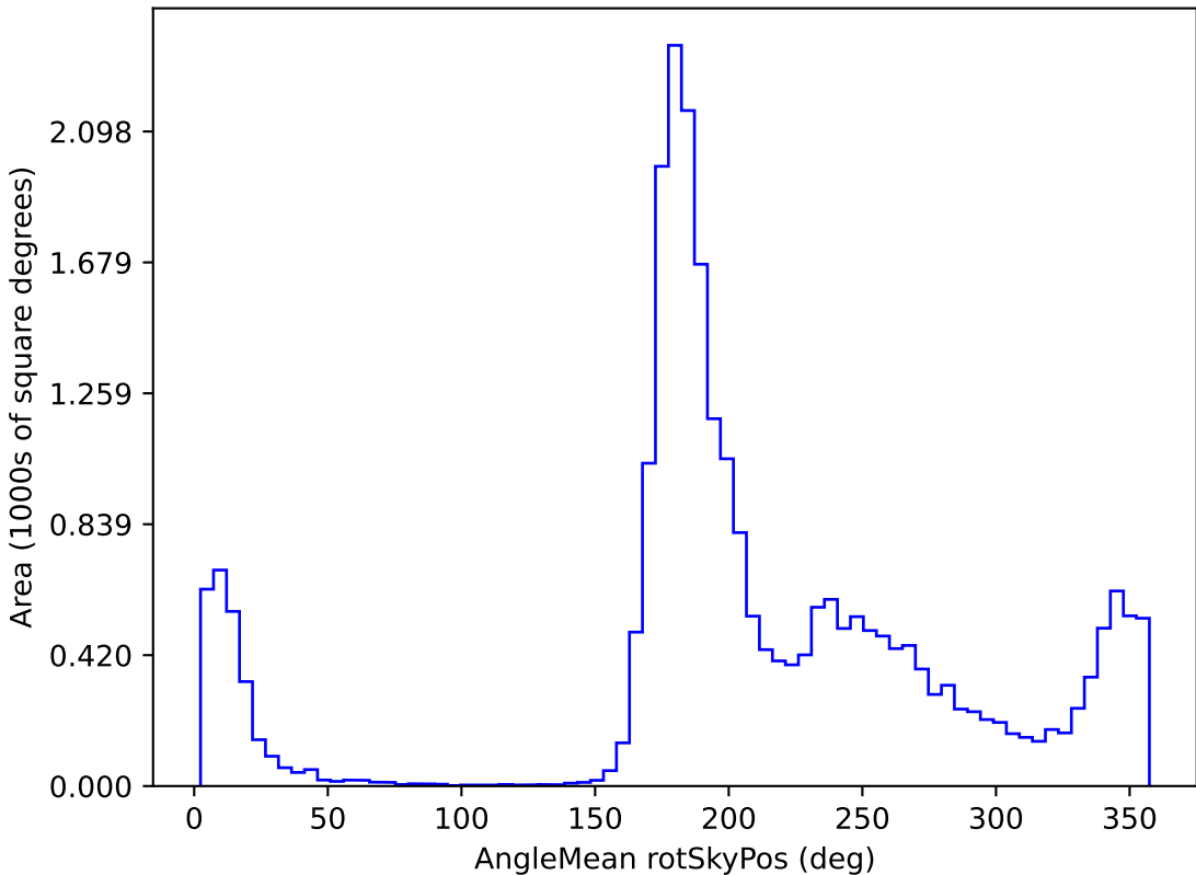
weather_cloudso1v3.4_10yrs All sky i band: AngleMean rotSkyPos
