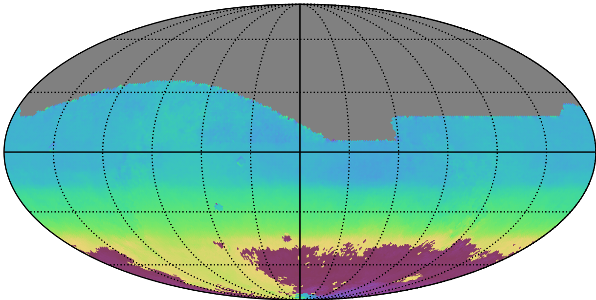
weather_cloudso1v3.4_10yrs All sky all bands: AngleMean rotSkyPos
