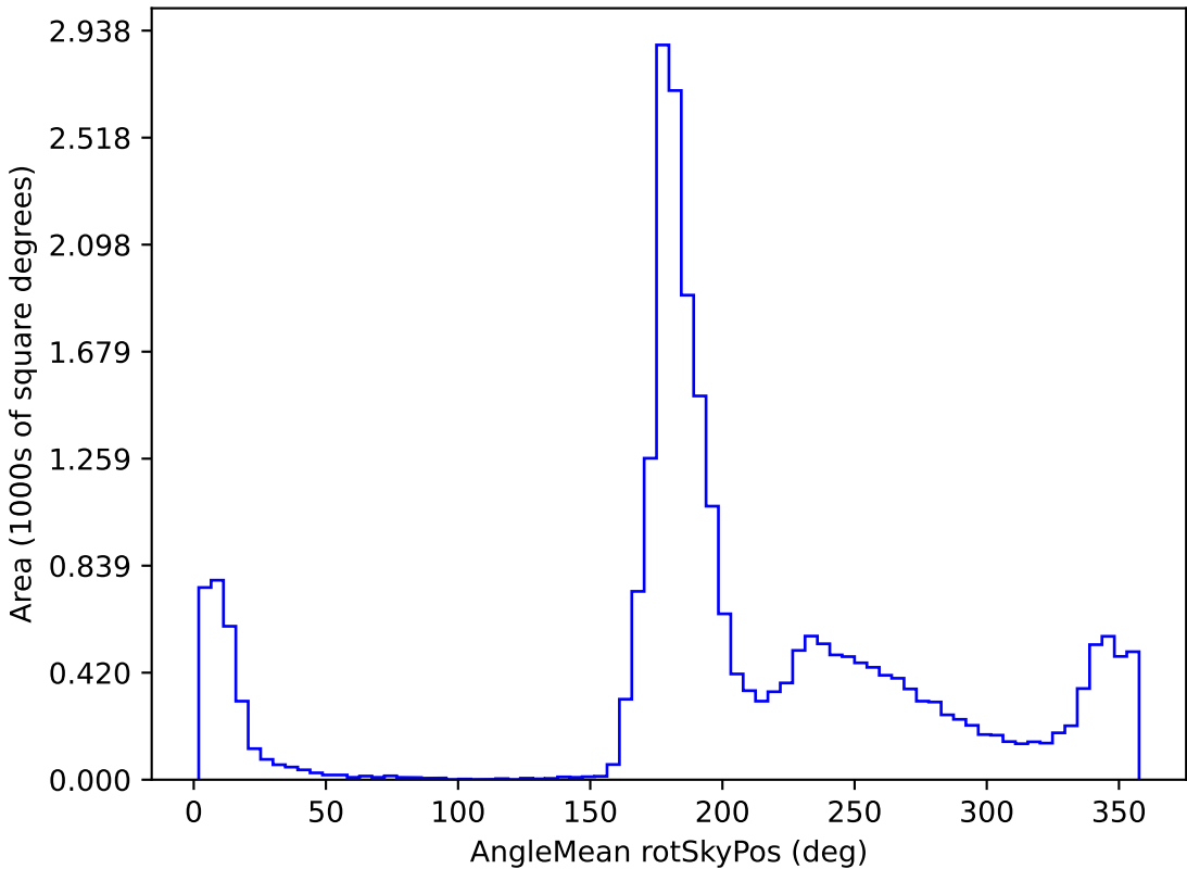
weather_cloudso1v3.4_10yrs All sky all bands: AngleMean rotSkyPos
