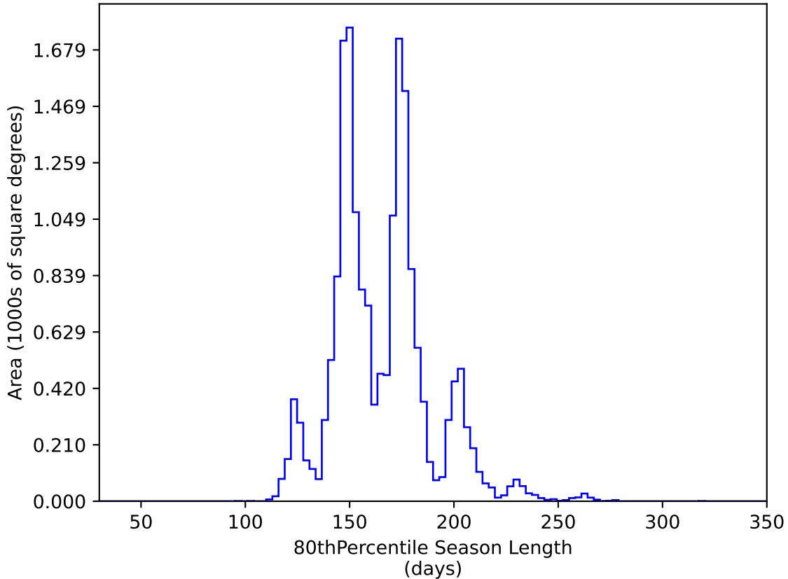
weather_cloudso1v3.4_10yrs WFD y band: 80thPercentile Season Length
