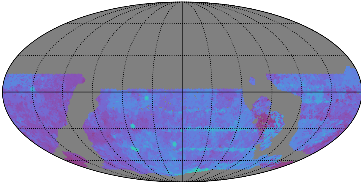
weather_cloudso1v3.4_10yrs WFD u band: 80thPercentile Season Length
