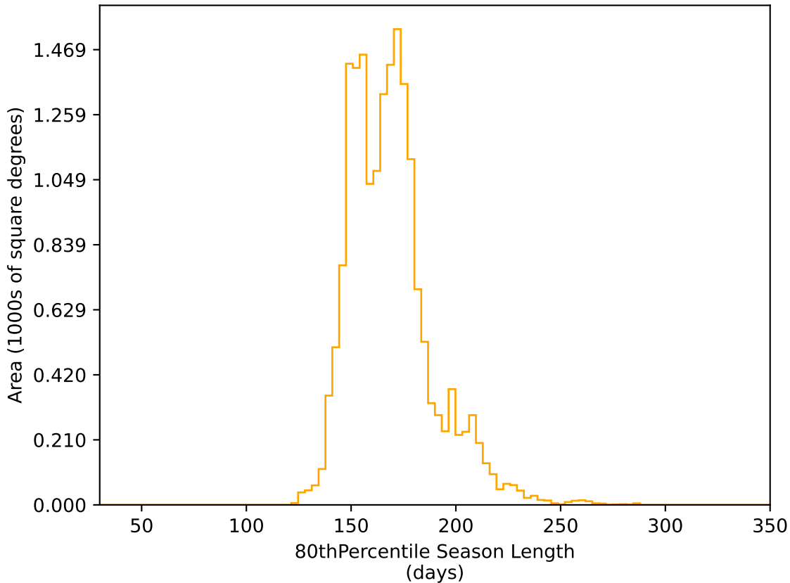
weather_cloudso1v3.4_10yrs WFD r band: 80thPercentile Season Length
