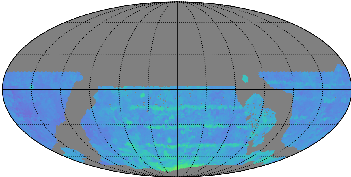
weather_cloudso1v3.4_10yrs WFD i band: 80thPercentile Season Length
