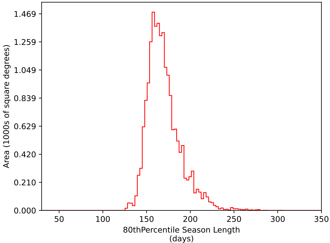
weather_cloudso1v3.4_10yrs WFD i band: 80thPercentile Season Length
