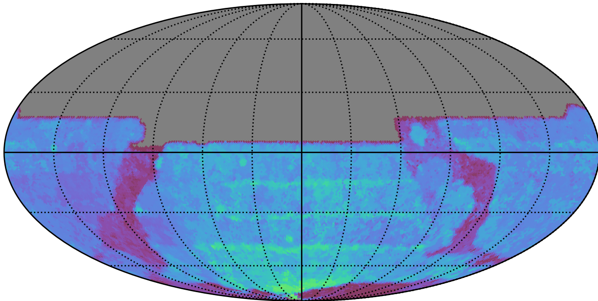
weather_cloudso1v3.4_10yrs All sky y band: 80thPercentile Season Length
