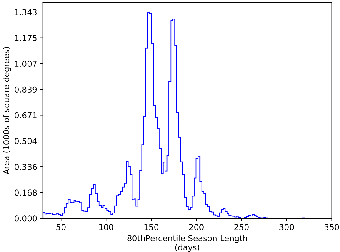
weather_cloudso1v3.4_10yrs All sky y band: 80thPercentile Season Length
