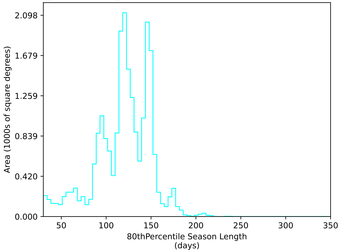
weather_cloudso1v3.4_10yrs All sky u band: 80thPercentile Season Length
