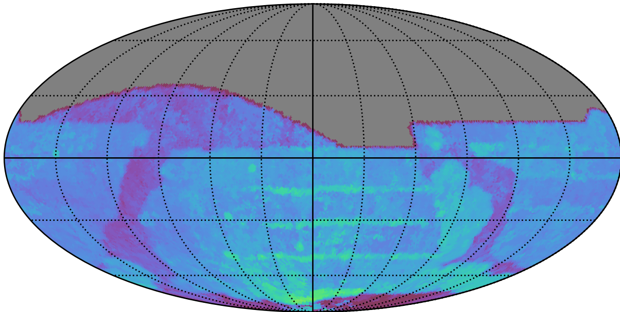
weather_cloudso1v3.4_10yrs All sky r band: 80thPercentile Season Length
