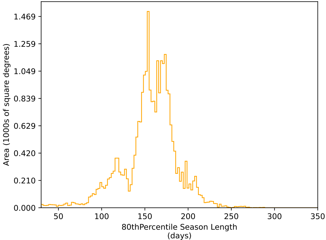
weather_cloudso1v3.4_10yrs All sky r band: 80thPercentile Season Length
