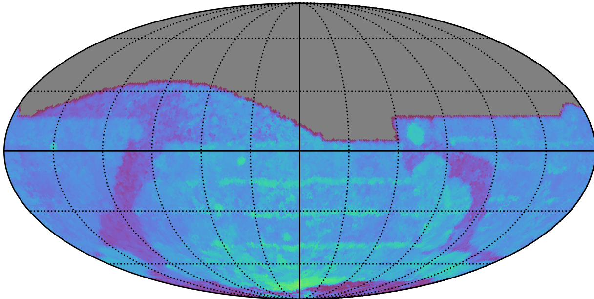
weather_cloudso1v3.4_10yrs All sky i band: 80thPercentile Season Length
