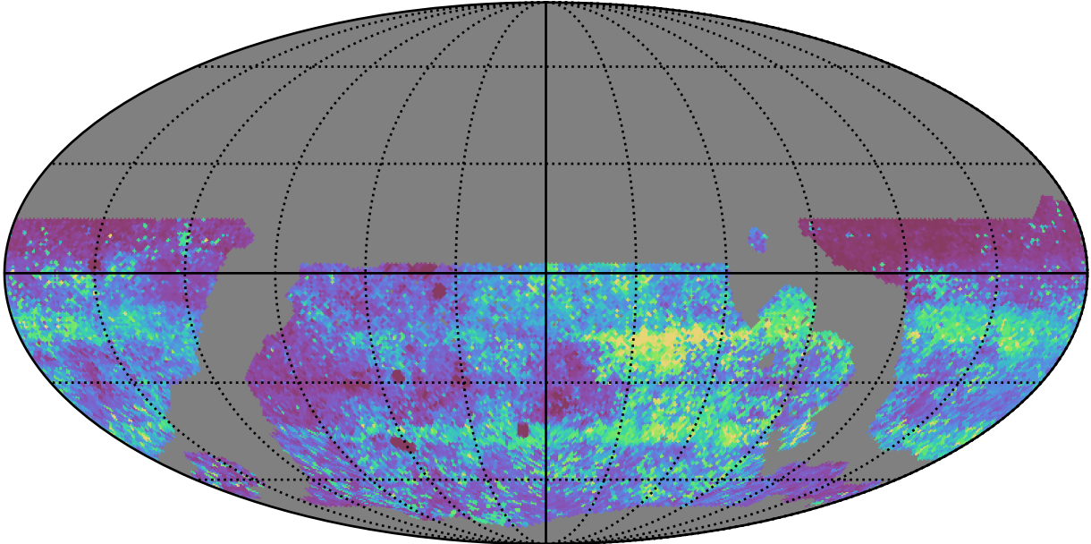
weather_cloudso1v3.4_10yrs WFD zy bands: 75th Percentile Intranight Timespan
