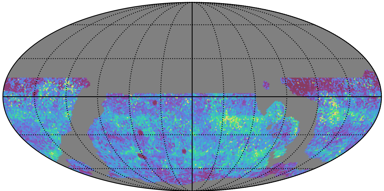
weather_cloudso1v3.4_10yrs WFD y band: 75th Percentile Intranight Timespan
