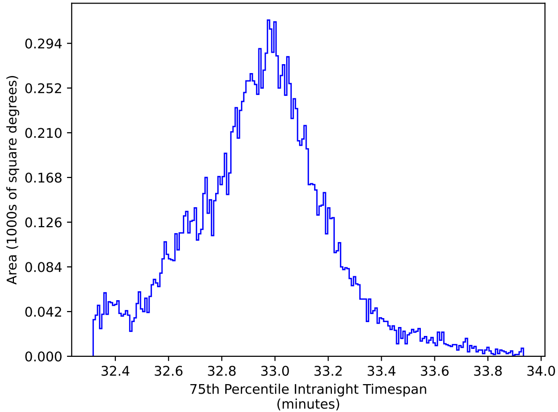
weather_cloudso1v3.4_10yrs WFD y band: 75th Percentile Intranight Timespan
