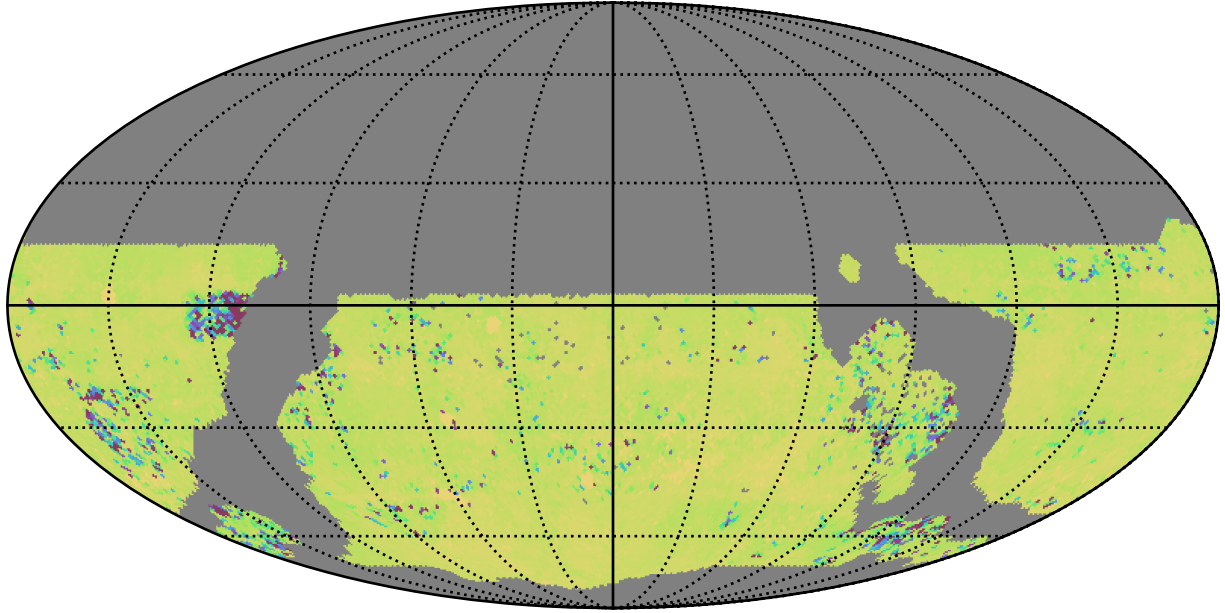
weather_cloudso1v3.4_10yrs WFD ug bands: 75th Percentile Intranight Timespan
