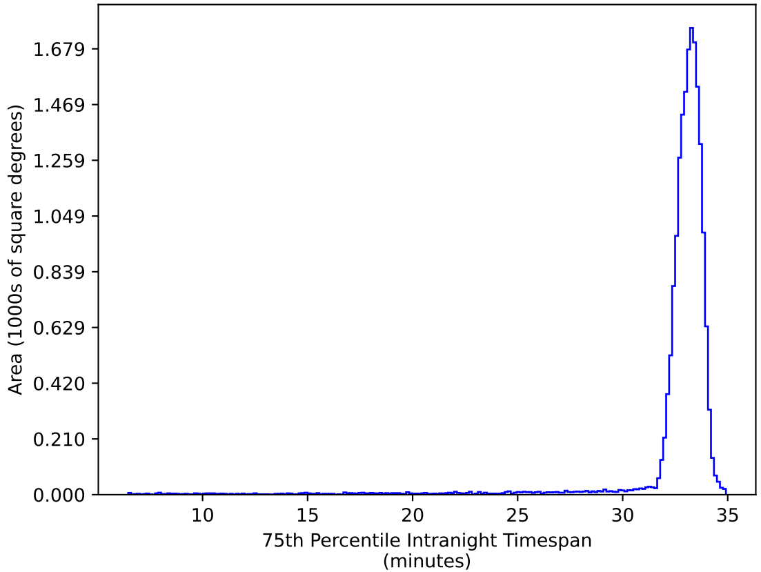
weather_cloudso1v3.4_10yrs WFD ug bands: 75th Percentile Intranight Timespan
