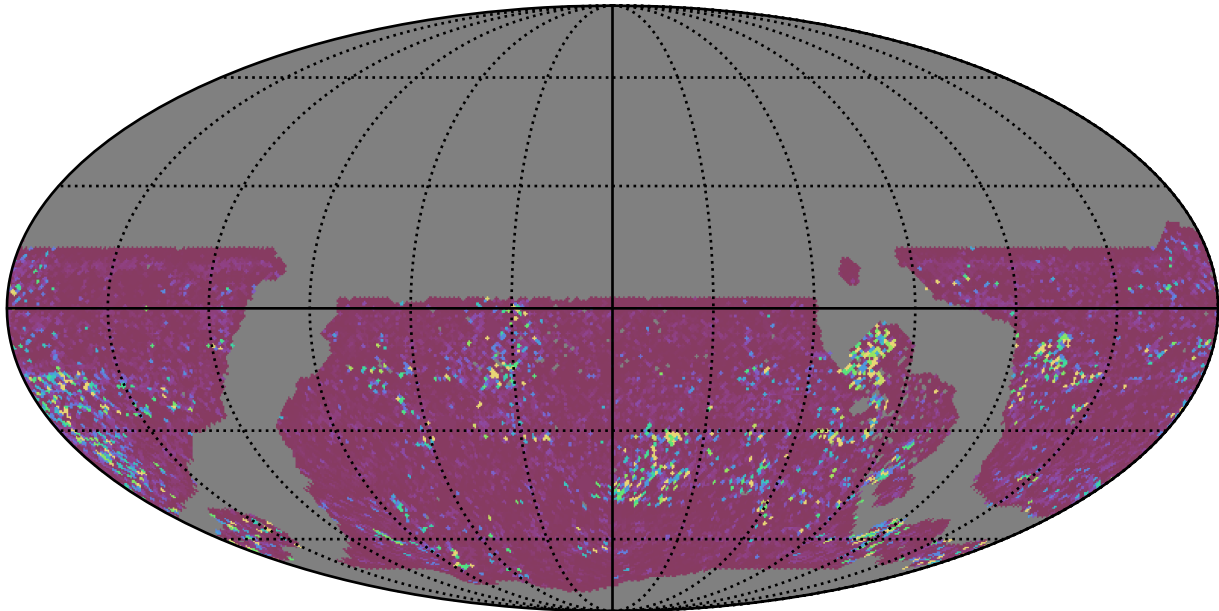
weather_cloudso1v3.4_10yrs WFD u band: 75th Percentile Intranight Timespan
