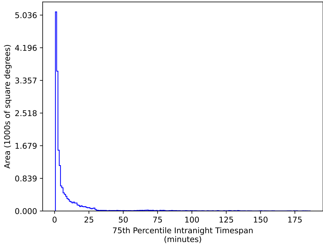
weather_cloudso1v3.4_10yrs WFD u band: 75th Percentile Intranight Timespan
