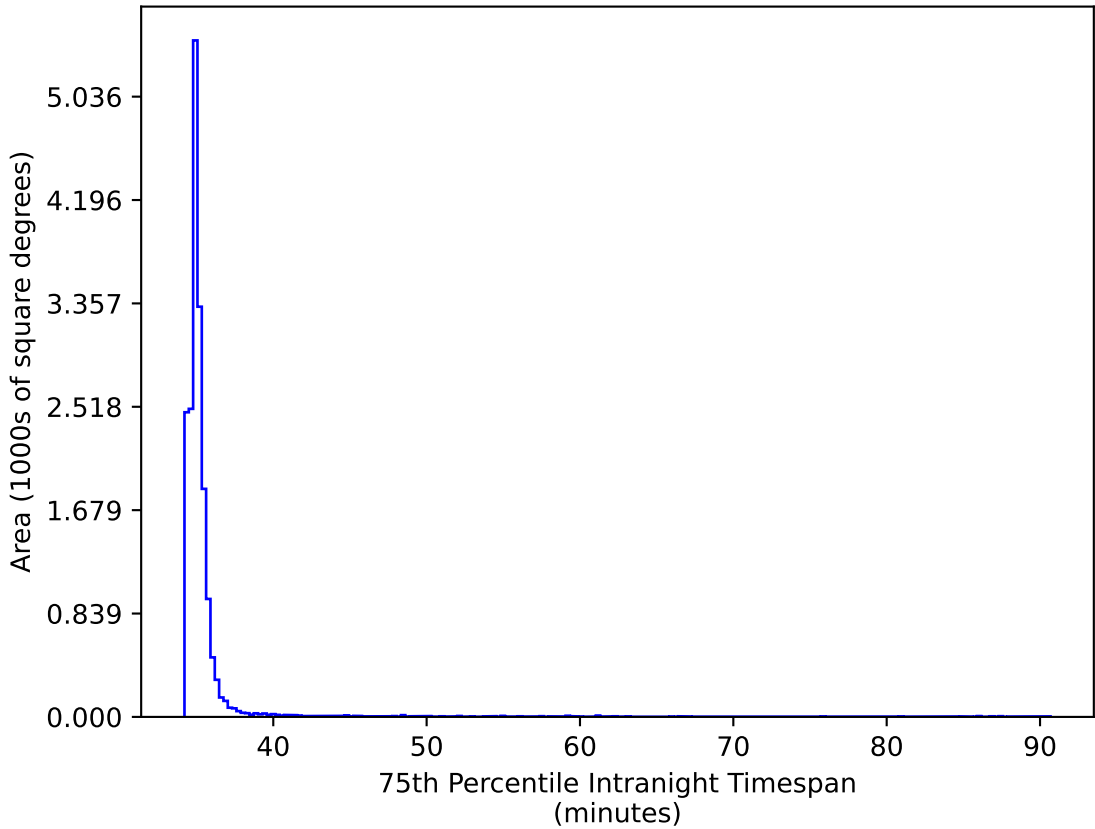
weather_cloudso1v3.4_10yrs WFD ri bands: 75th Percentile Intranight Timespan
