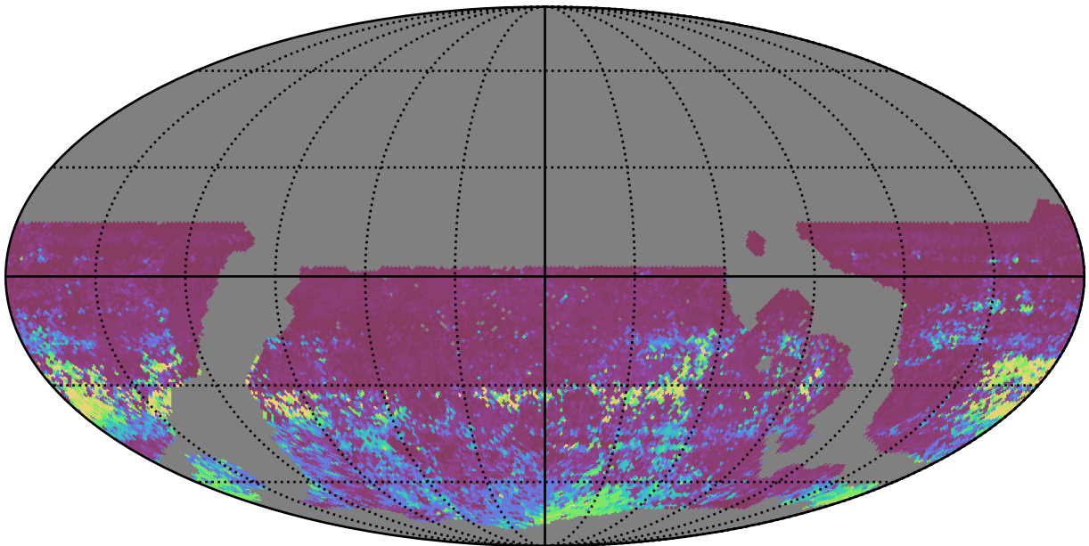
weather_cloudso1v3.4_10yrs WFD r band: 75th Percentile Intranight Timespan
