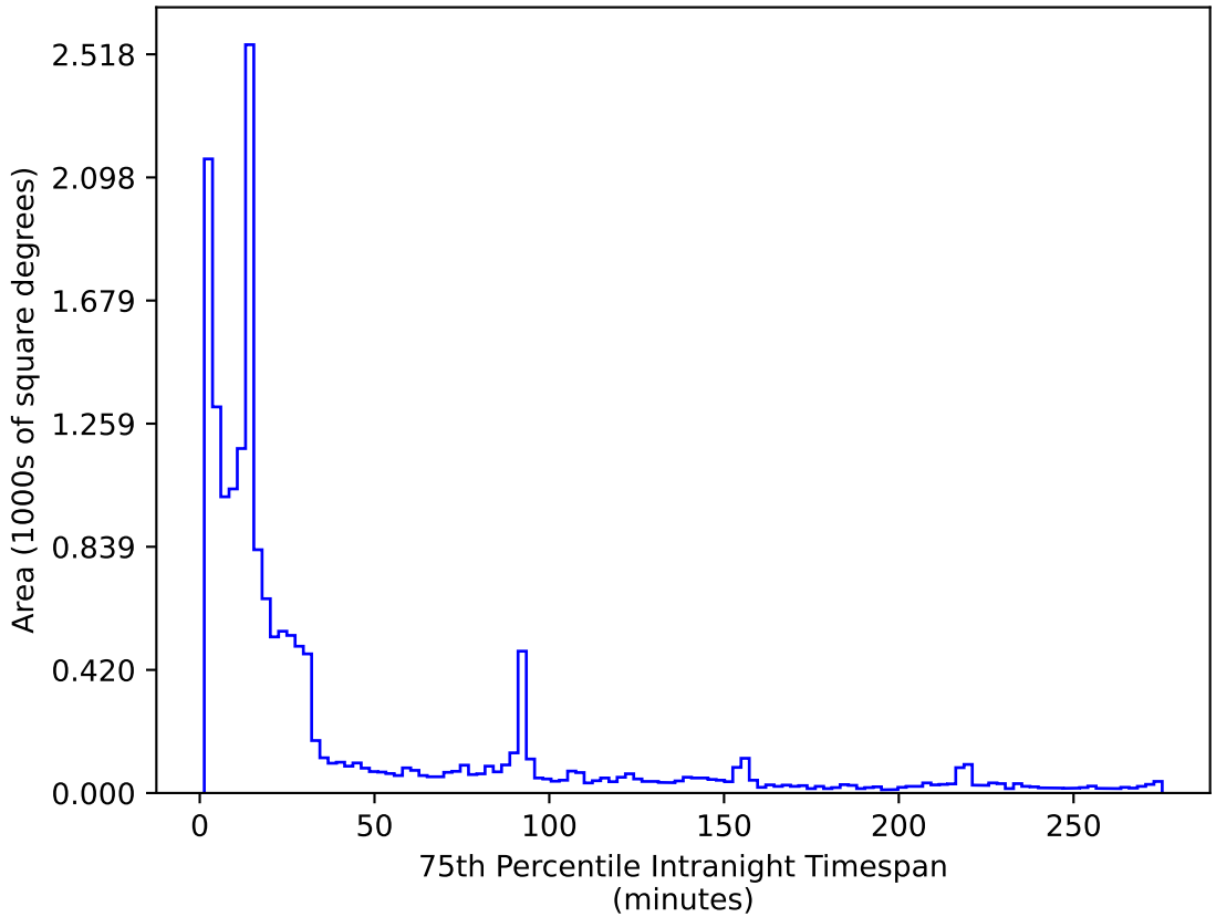
weather_cloudso1v3.4_10yrs WFD r band: 75th Percentile Intranight Timespan
