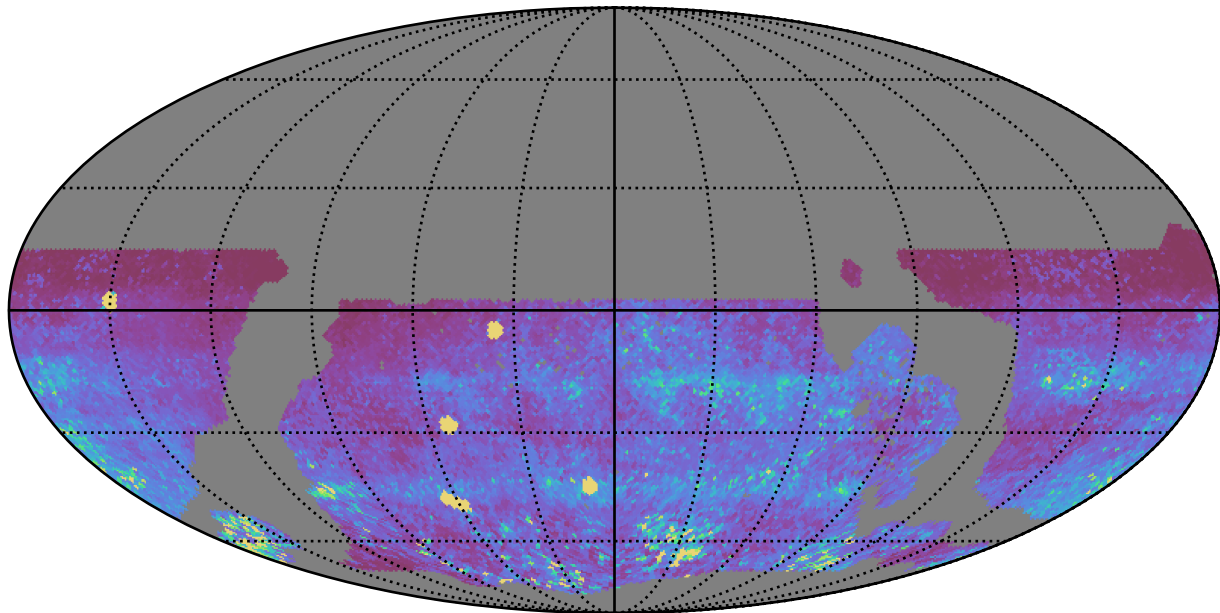
weather_cloudso1v3.4_10yrs WFD iz bands: 75th Percentile Intranight Timespan
