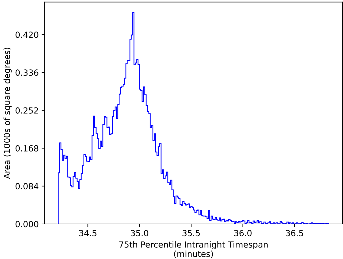
weather_cloudso1v3.4_10yrs WFD iz bands: 75th Percentile Intranight Timespan
