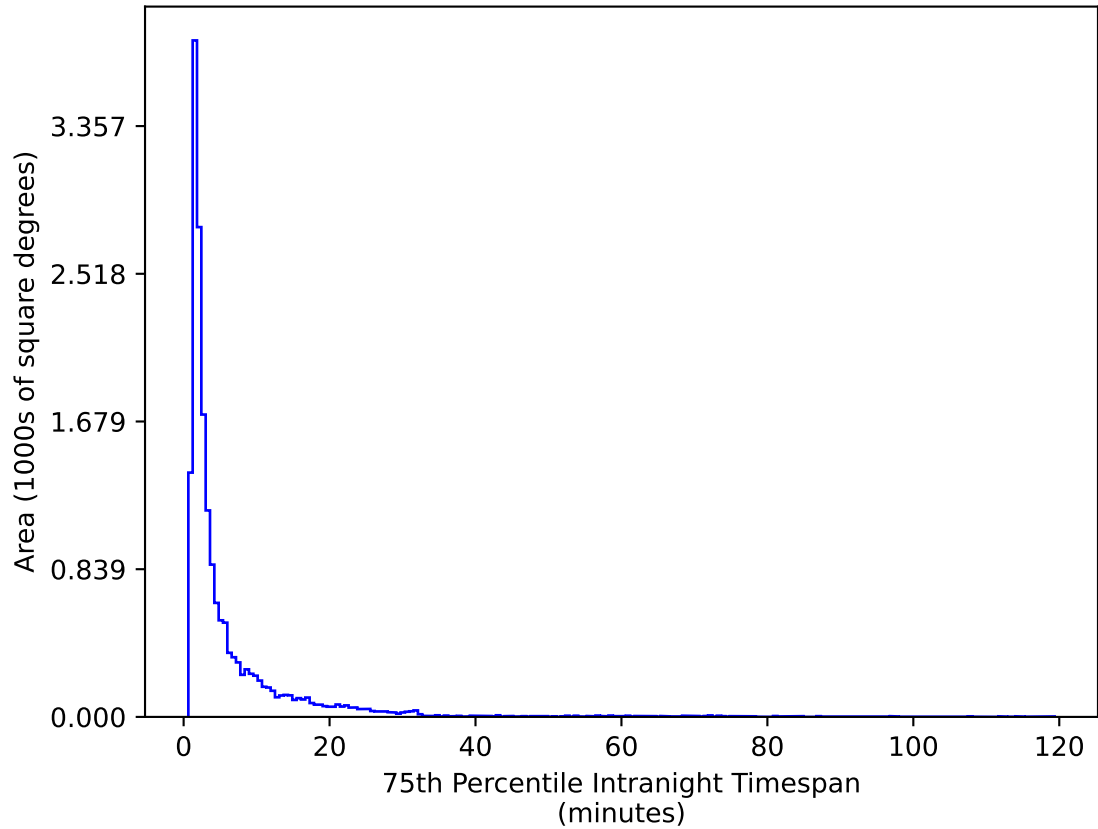
weather_cloudso1v3.4_10yrs WFD g band: 75th Percentile Intranight Timespan
