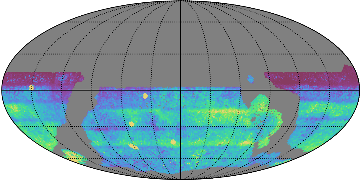
weather_cloudso1v3.4_10yrs WFD all bands: 75th Percentile Intranight Timespan
