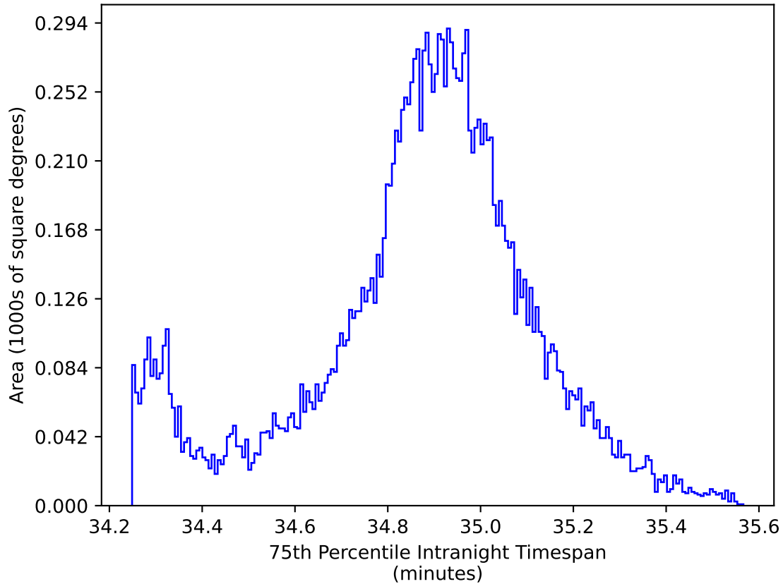
weather_cloudso1v3.4_10yrs WFD all bands: 75th Percentile Intranight Timespan
