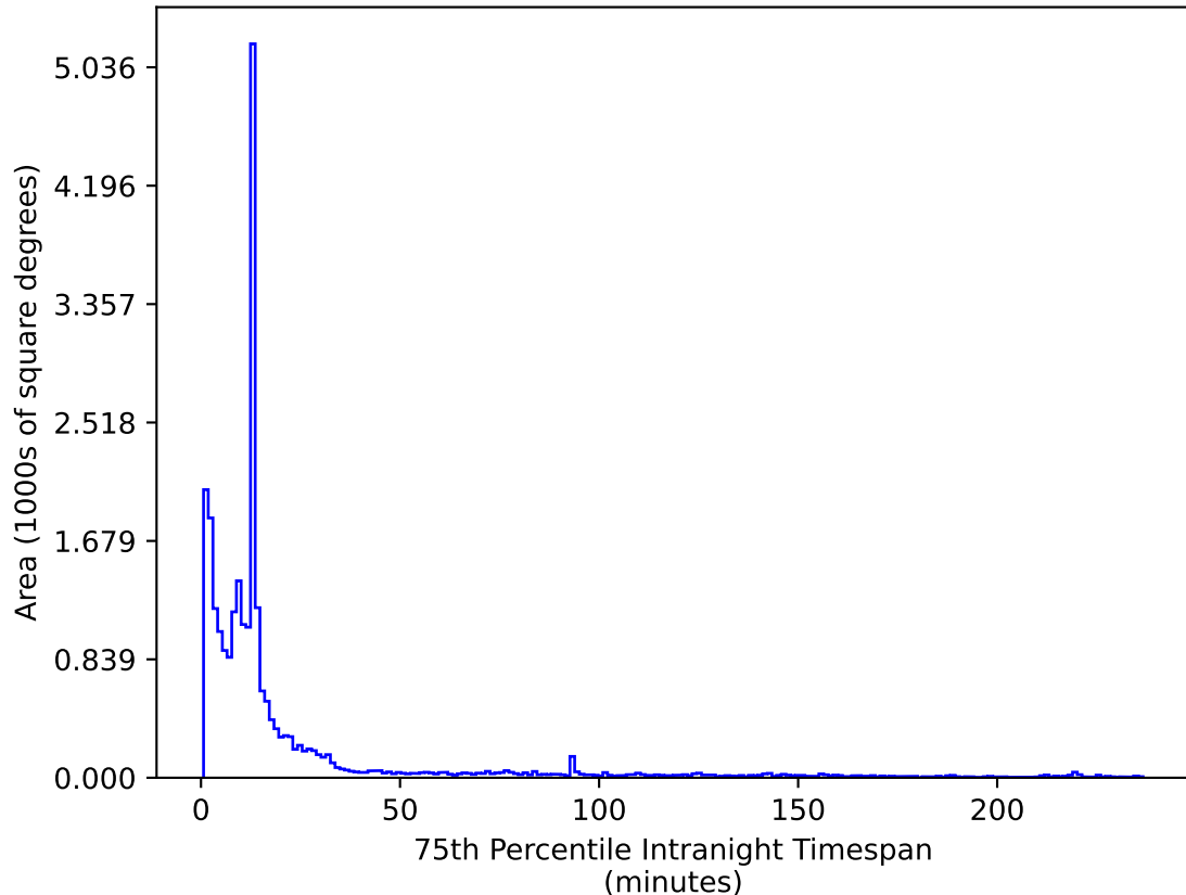
weather_cloudso1v3.4_10yrs All sky z band: 75th Percentile Intranight Timespan
