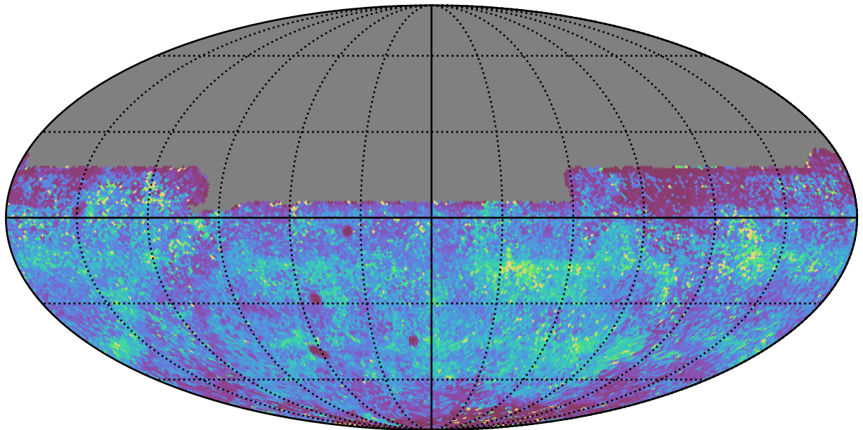
weather_cloudso1v3.4_10yrs All sky y band: 75th Percentile Intranight Timespan
