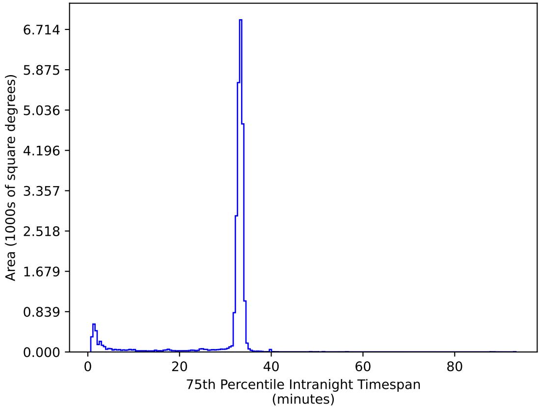
weather_cloudso1v3.4_10yrs All sky ug bands: 75th Percentile Intranight Timespan
