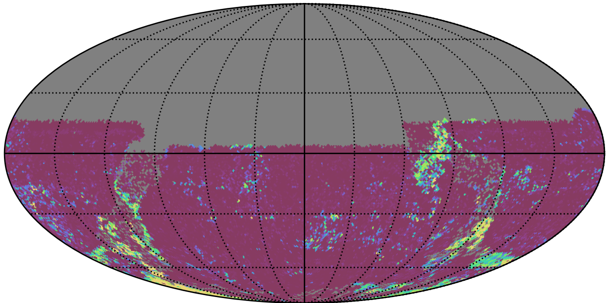
weather_cloudso1v3.4_10yrs All sky u band: 75th Percentile Intranight Timespan
