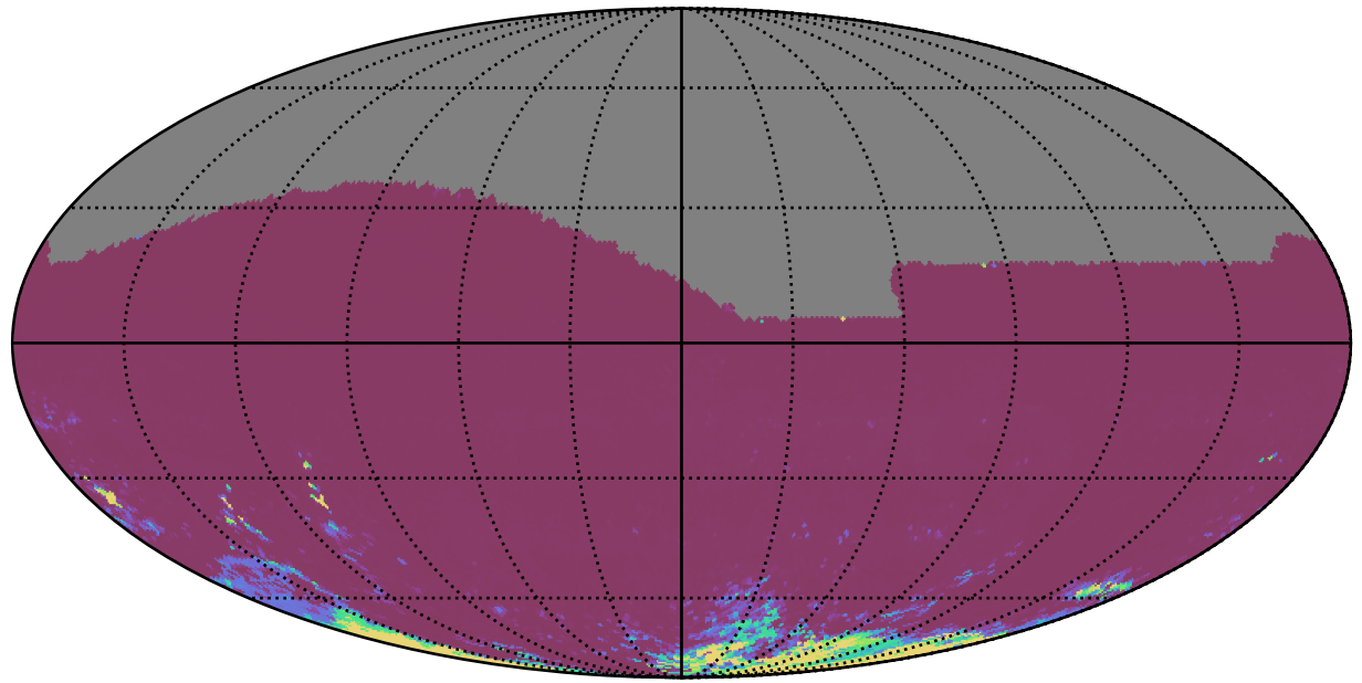
weather_cloudso1v3.4_10yrs All sky ri bands: 75th Percentile Intranight Timespan
