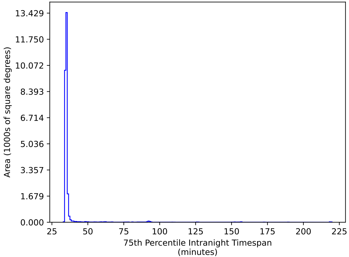
weather_cloudso1v3.4_10yrs All sky ri bands: 75th Percentile Intranight Timespan
