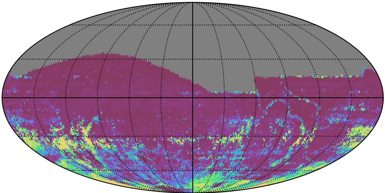
weather_cloudso1v3.4_10yrs All sky r band: 75th Percentile Intranight Timespan
