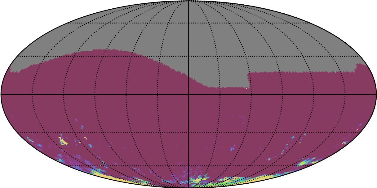
weather_cloudso1v3.4_10yrs All sky gr bands: 75th Percentile Intranight Timespan
