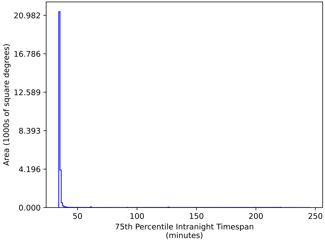
weather_cloudso1v3.4_10yrs All sky gr bands: 75th Percentile Intranight Timespan
