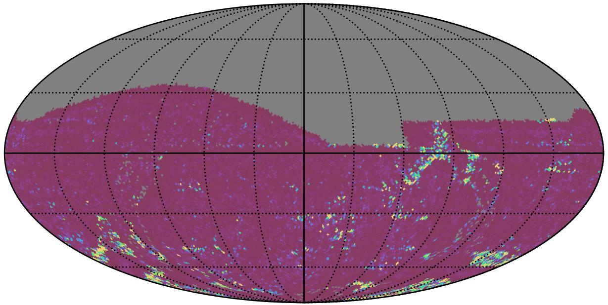
weather_cloudso1v3.4_10yrs All sky g band: 75th Percentile Intranight Timespan
