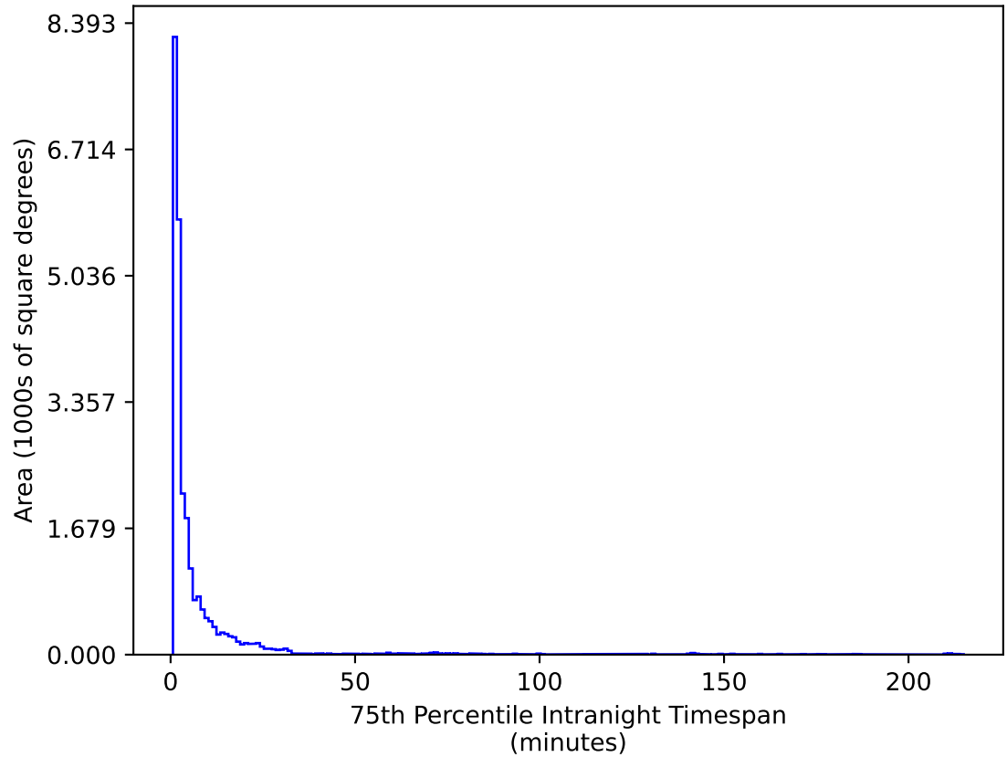
weather_cloudso1v3.4_10yrs All sky g band: 75th Percentile Intranight Timespan
