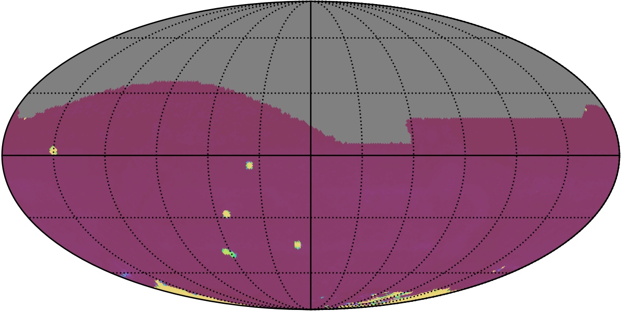
weather_cloudso1v3.4_10yrs All sky all bands: 75th Percentile Intranight Timespan
