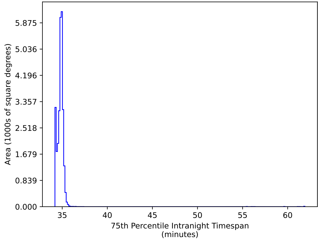
weather_cloudso1v3.4_10yrs All sky all bands: 75th Percentile Intranight Timespan
