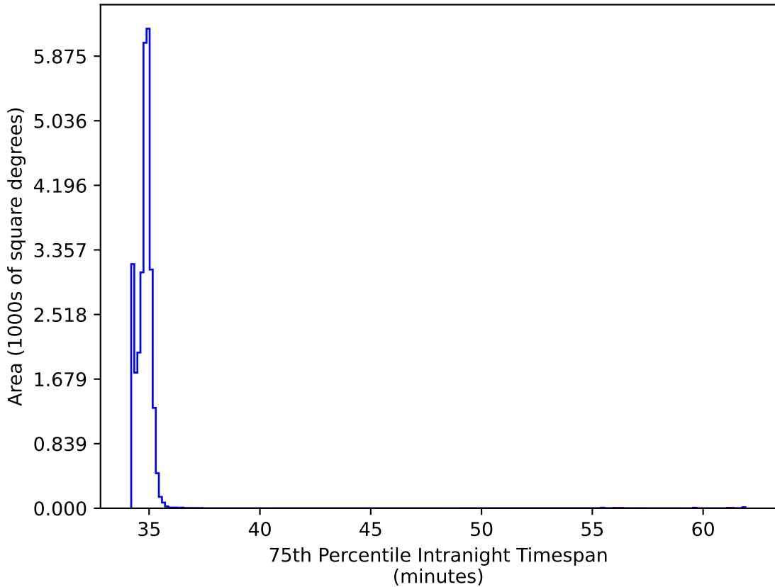
weather_cloudso1v3.4_10yrs All sky: 75th Percentile Intranight Timespan
